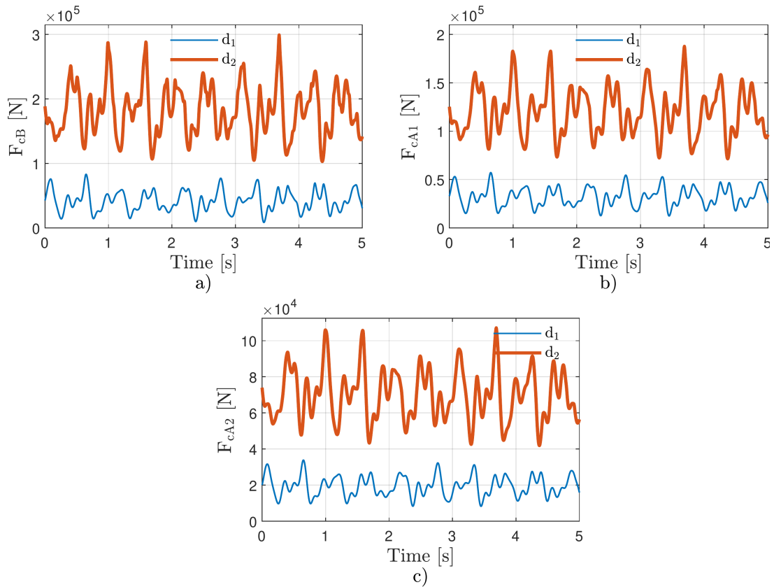
Fig. 13. Variation in the driving force of (a) the boom cylinder F_{cB} , (b) the arm #1 cylinder F_{cA1} , and (c) the arm #2 cylinder F_{cA2}
