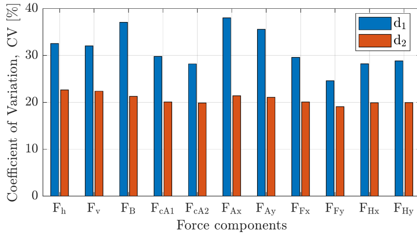
Fig. 15. Coefficient of variation of the force components for two cutting depths
