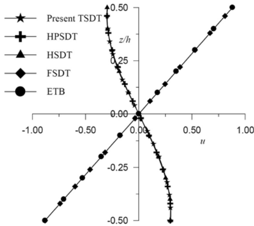
Fig. 3. Variation of axial displacement ( \bar{u} ) through the thickness of fixed-fixed beam at ( x = 0.75L , z ) for slenderness ratio 4
