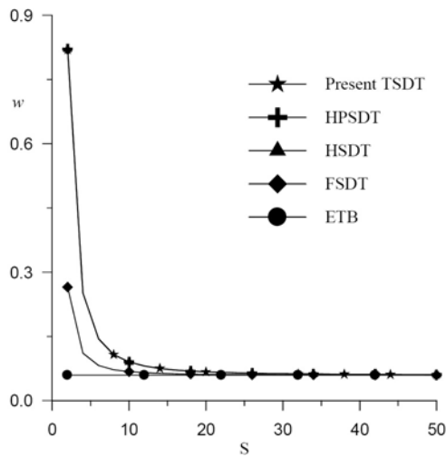
Fig. 5. Variation of maximum transverse displacement ( \bar{w} ) of fixed-fixed beam at ( x = 0.75L , z = 0 ) with slenderness ratio S
