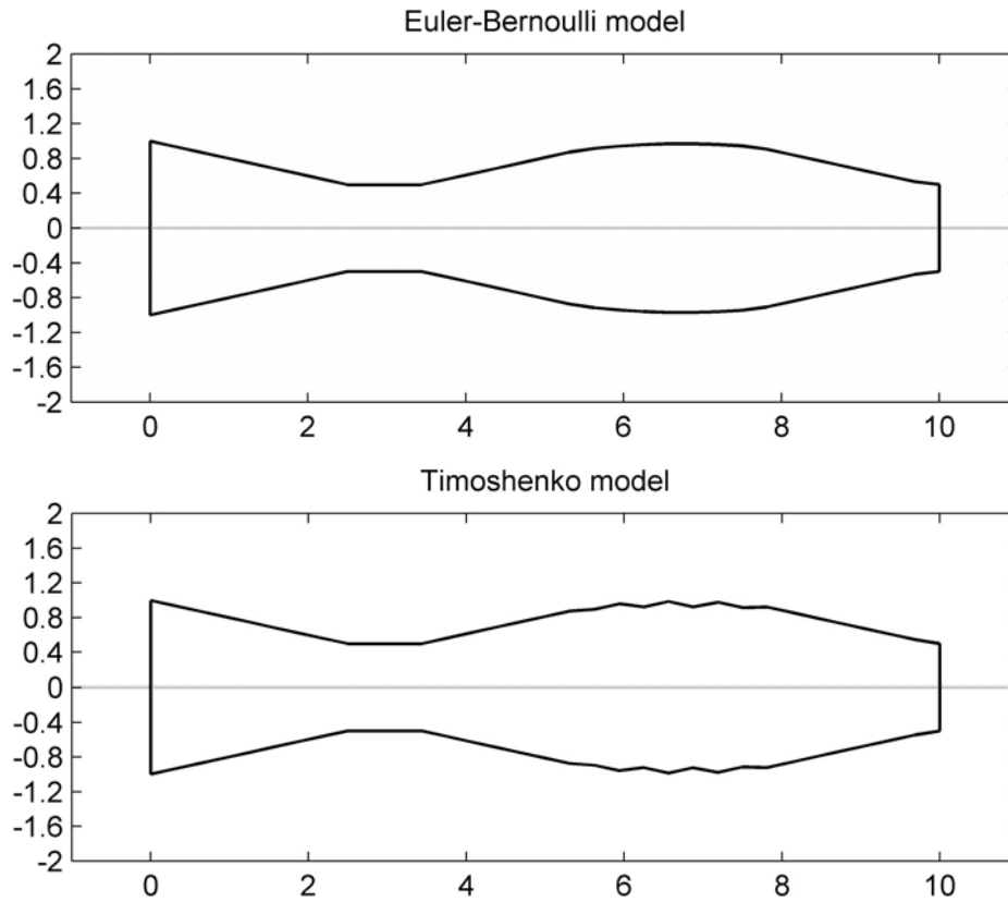
Fig. 1. An optimal thickness with respect to the compliance cost functional
