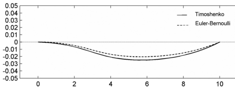
Fig. 2. A deflection of the optimal beam
