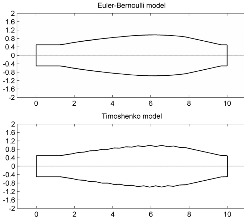
Fig. 3. A beam minimizing the compliance
