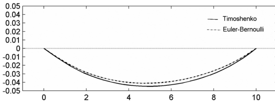
Fig. 4. A deflection of the beam with optimal thickness
