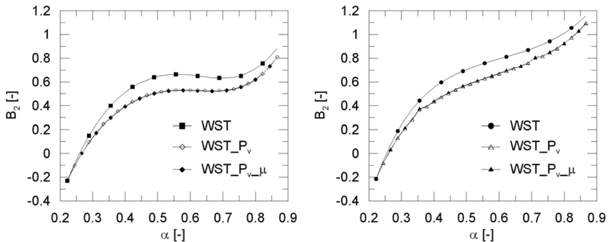
Fig. 8. Normalized values of the T -stress, B_2 , for cube-shaped (left) and cylinder-shaped (right) WST specimen
