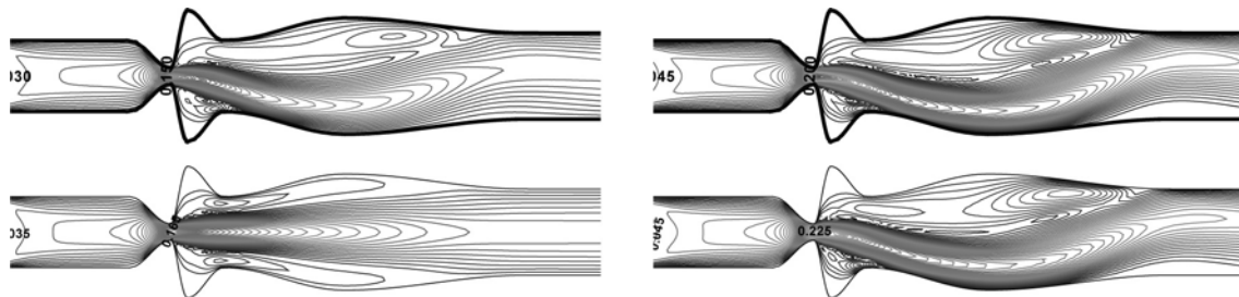
Fig. 4. The isolines of flow velocity magnitudes for Reynolds number 50 (left) and 70 (right) on isotropic mesh(upper part) and anisotropic mesh (lower part)
