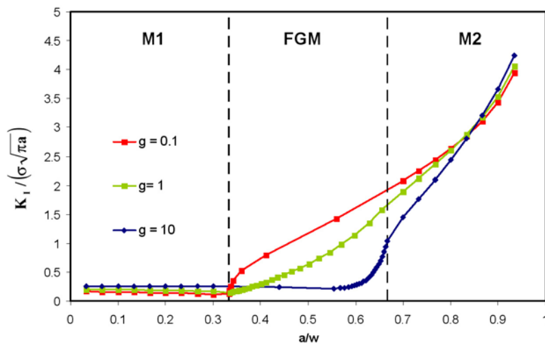
Fig. 9. Stress intensity factors E_2/E_1 = 10 , displacement loading
