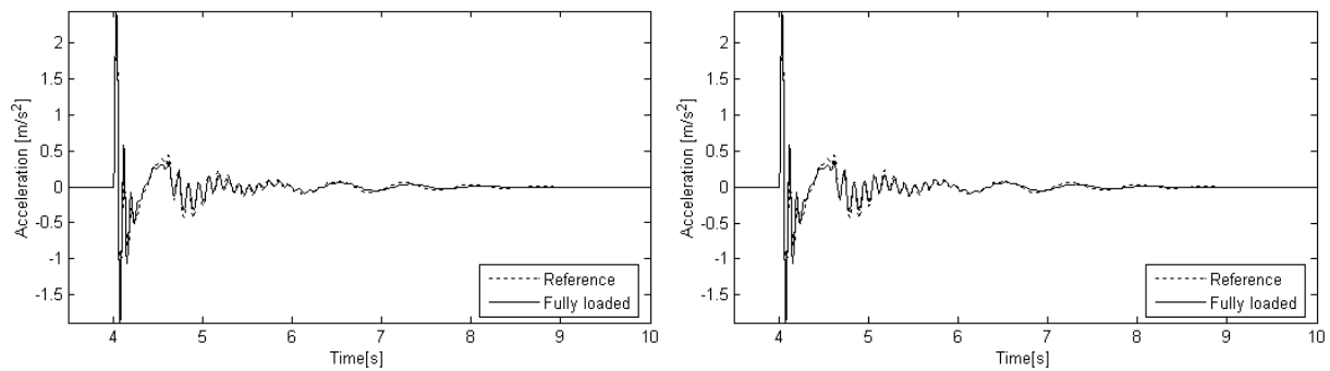
Fig. 7. Time histories of the vertical acceleration at the chassis under the driver's seat of the fully loaded bus and of the bus of the reference load (comparison of the reference case with the original, i.e. after the optimization of the front APCSA, and optimally tuned force-velocity characteristics after the optimization of the rear APCSA).
